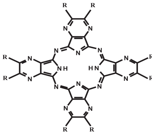
Structure of tetrapyrzinoporphyrazine R = \text{C}_2\text{H}_5 ( I ), R = \text{C}_6\text{H}_5 ( II )
